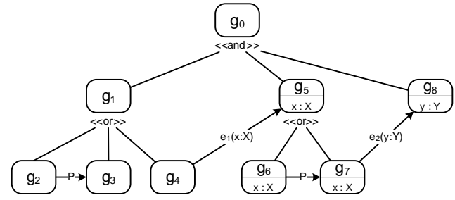
Figure 2: Specification Tree with Precedence
