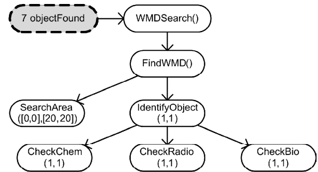
Figure 9: IdentifyObject Triggered at 1,1
