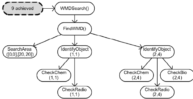
Figure 11: CheckBio(1,1) is Achieved
