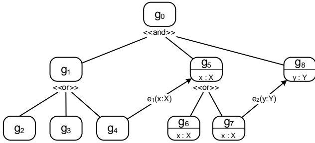
Figure 1: Goal Specification Tree
