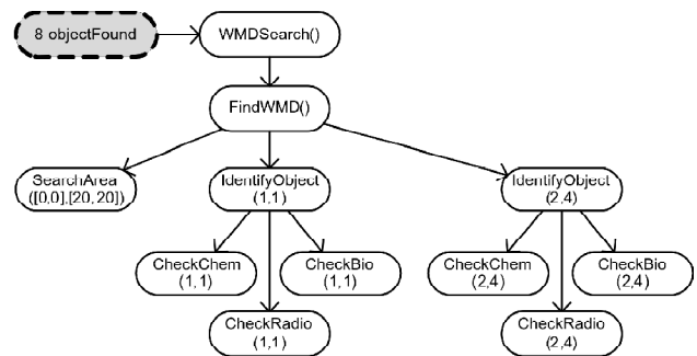
Figure 10: IdentifyObject Triggered at 2,4
