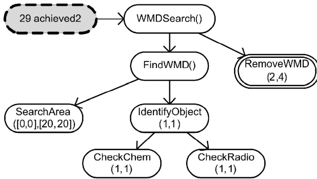
Figure 12: RemoveWMD Goal Created
