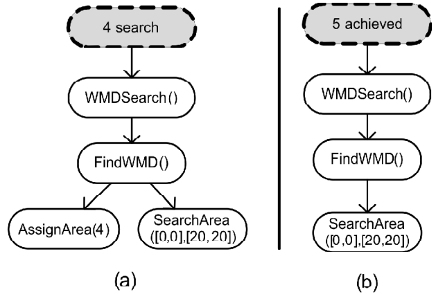
Figure 8: Search and Achieve Events
