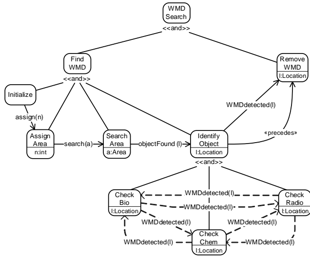
Figure 6: WMD Goal Specification Tree
