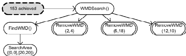
Figure 13: No More IdentifyObject Goals
