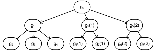
Figure 5: G_{Instance} Tree after Second e_1 Event
