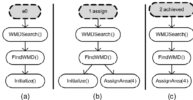
Figure 7: Initial, Assign, and Achieve Events
